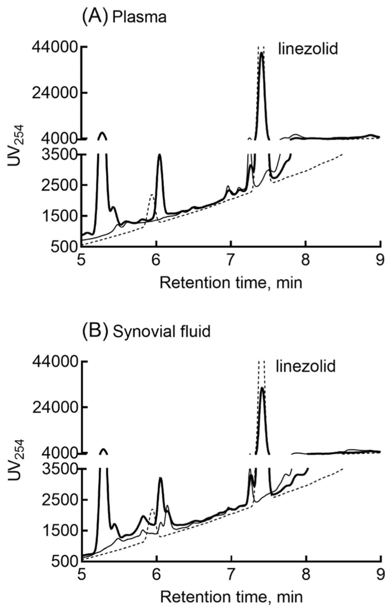
Fig. 2 Representative chromatograms for linezolid in plasma and linezolid in synovial fluid. Plasma (A) and synovial fluid (B) samples from case 1 before (thin lines) and after (thick lines) treatment with linezolid twice a day were investigated. Possible linezolid 2-hydroxylated metabolite(s) mediated by recombinant human P450 2J2 in an in vitro system (dashed lines) was used for chromatographic comparison. The retention times of linezolid and its possible 2-hydroxylated metabolite [9] were 7.4 and 5.9 min respectively
