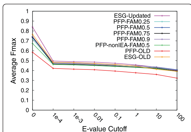
Fig. 2 Performance of PFP and extended similarity group (ESG) on GO terms including parental terms. Each predicted and true GO term was propagated to the root of the ontology before evaluation. GO terms in all three ontologies (BP, MF, CC) were used in computing prediction accuracy
