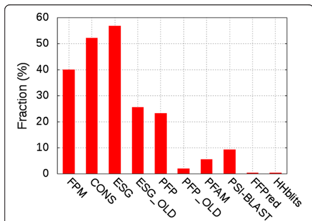
Fig. 3 Fraction of queries where each method showed the largest F_{max} score. The fraction on the y-axis was computed as the number of queries in which a method had the largest F_{max} score over the total number of queries (2,055 protein sequences). Frequent pattern mining (FPM) in this graph denotes FPM_MaxLen because it performed better than its counterpart, FPM_maxscoreLen. The fraction does not sum up to 100 % because there were cases where multiple methods tied for the largest F_{max} score
