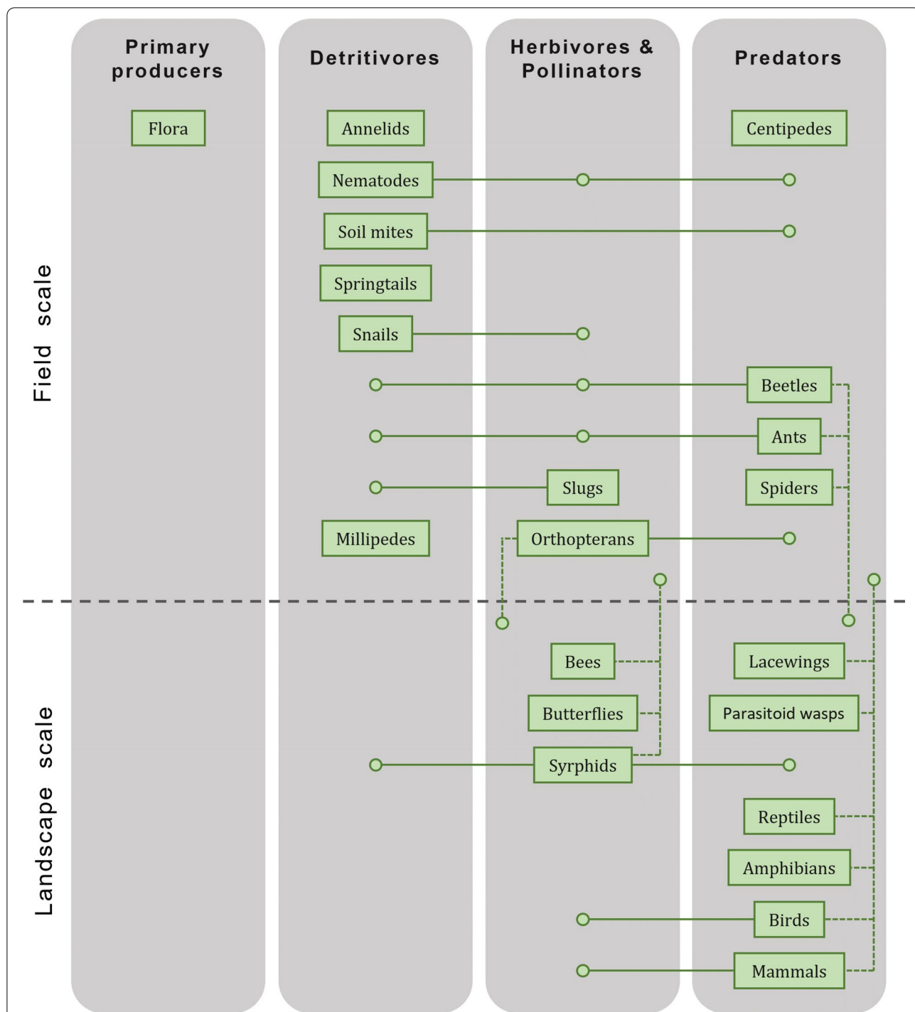
Fig. 1 Indicator species groups (ISGs). Representation of the twenty-two ISGs selected for the systematic map based on their trophic level (vertically) and scale of indication (horizontally). Among an ISG, these two parameters might differ between species or stages of development (i.e., larva or adult), so the main classification is indicated by its name in a rectangle, and the other possibilities by a dot connected with a line (plain to indicate possible variations in trophic level and dashed in the scale of indication). These classifications are not exhaustive and are primarily intended to provide an overview of the different ISGs. Adapted from Fig. 6.1 in [19]
