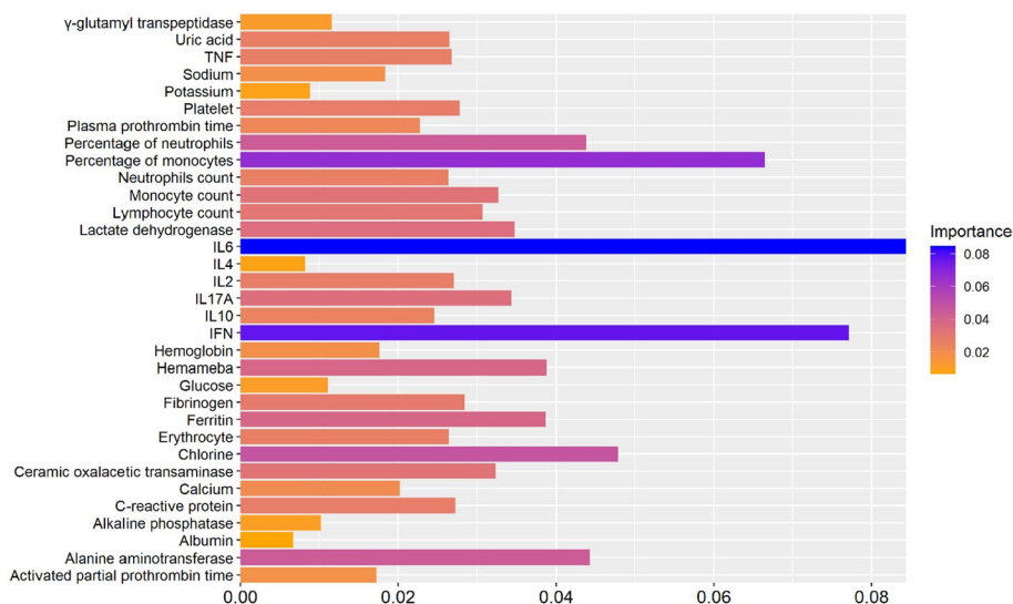
Fig. 3 The XGBoost algorithm ranks the features importance of the features data used to predict CRS
