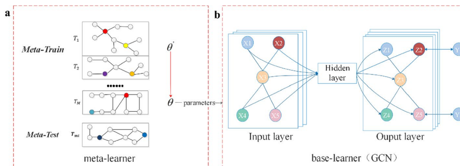
Fig. 1 Meta-GNN is composed of two modules. a Meta-learner module can optimize the initial training parameters of the model. b Base-learner module is GCN model
