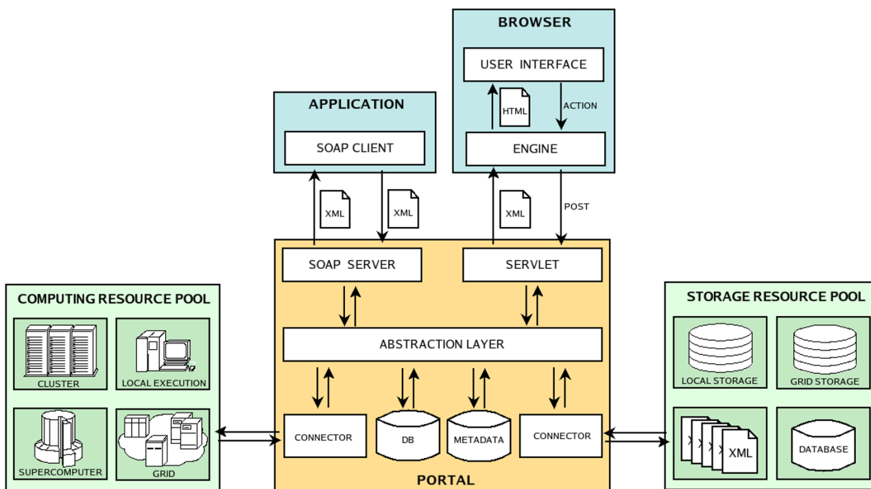
Figure 2 Architectural design of the portal.
