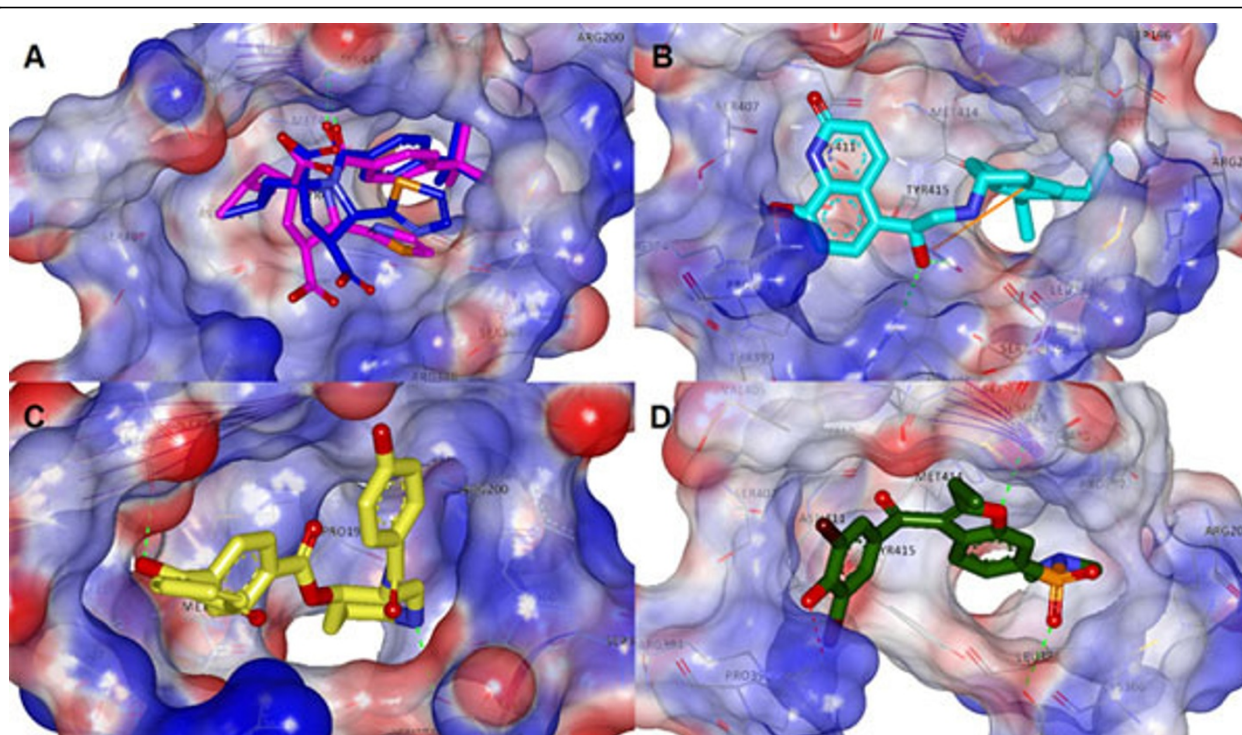
Figure 6 A) Overlay of docked and PDB coordinates of 2JC1 ligand for the Palm I site (original ligand pose coloured blue, docked ligand pose coloured pink); B) docked pose of DB05039 it shows a very good placement of the diethyl-indanyl group into the deep pocket. A salt bridge strengthens the binding with ARG394. Similarly, hydrogen bonding with ARG386 and TYR415, and Pi stacking with TYR415; C) docked pose of DB01940 forming a HB inside the deep hydrophobic pocket (as with one of benzodiazepines) in addition to a HB with GLN446 (just four atoms away along the backbone's TYR448 amidic nitrogen); D) docked pose of DB04142.(red dotted lines represent salt bridges, green dotted lines represent hydrogen bonds, orange solid lines represent \pi -interactions, backbone shown as curved purple lines, protein transparent surface with interpolated charges; bluish(+ve), reddish(-ve)). The furan ring show similar interaction with TYR448. These three hits preserved these binding modalities after molecular dynamics simulations.
