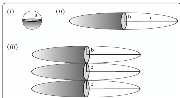
Figure 3 Shapes of macromolecules and lateral association orientation. The figures (i) and (ii) show the two different plausible shapes used to represent the protofibrils along with their appropriate dimensions. In the past these molecules have been represented as spheres for the most part. Based on experimental observations we suggest that a prolate spheroidal shape is more appropriate. Figure (iii) indicates the association mechanism of two spheroidal molecules. Since the ratio \frac{b}{c} \ll 1 , we can effectively assume that the association of two spheroids creates another spheroid with major and minor axes c and 2b , respectively.
