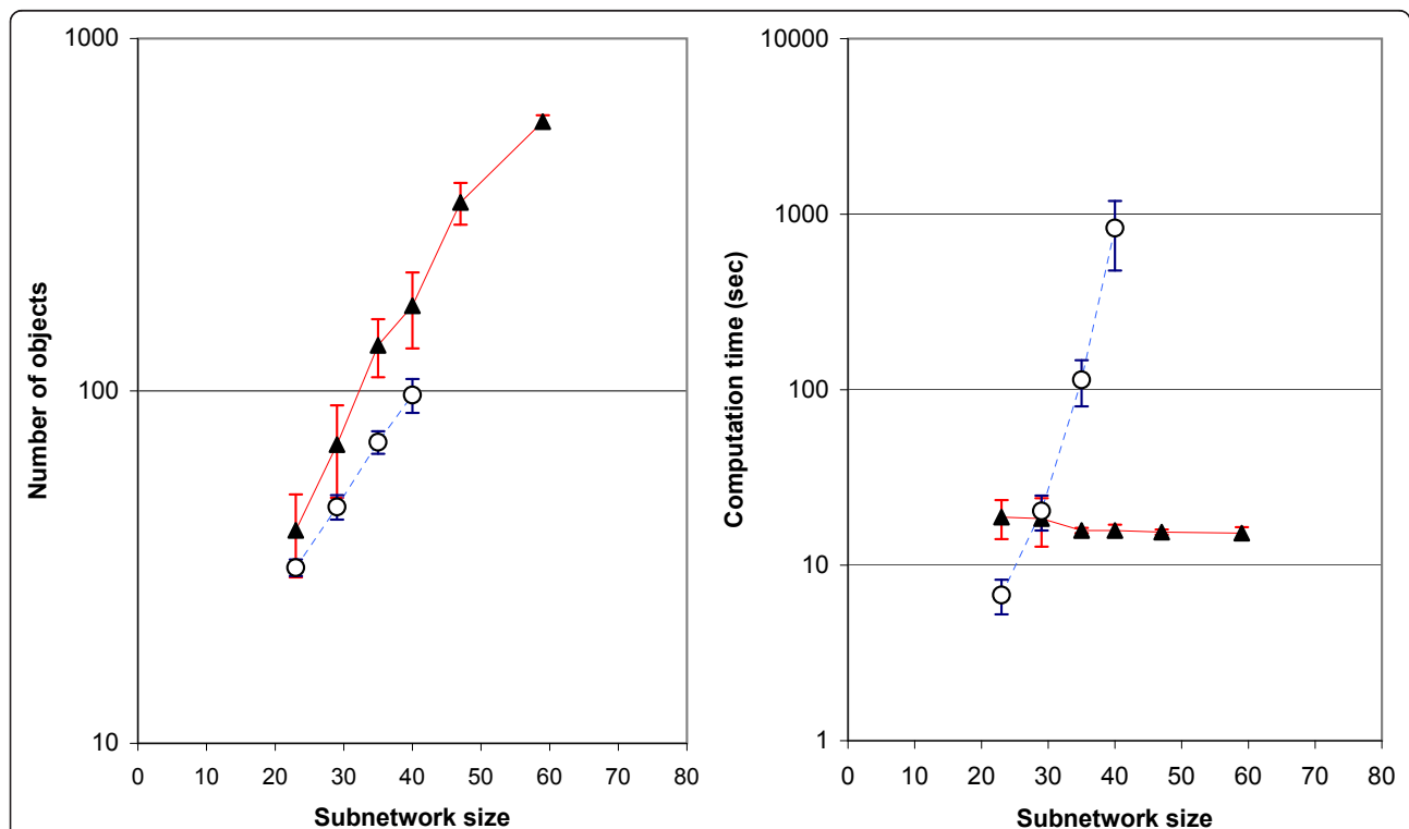
Figure 3 ProCEM vs. EFP computation. Left: Number of ProCEMs and EFPs computed for random subnetworks of different sizes. Right: The computation times (per second) required for computing the ProCEMs and EFPs in the left chart. \blacktriangle : ProCEMs; \circ : EFPs. Each experiment is repeated 100 times. Confidence intervals in this plot are based on one-sample t -test (95% c.i.). For large subnetworks ( r > 40 ), we did not compute the EFPs because the program was very slow.
