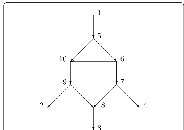
Figure 3 This tree-child network has X = \{1, 2, 3, 4\} . There are 7 arcs not leading to a hybrid vertex but only 6 distances, and the weights are not uniquely determined. The network is not normal because arc (5, 10) is redundant.
