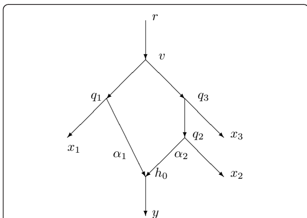
Figure 2 A minimal configuration needed to be able to find the probability \alpha_1 = \alpha(q_1, h_0) = 1 - \alpha_2 that a character state in h_0 is inherited from q_1 .
